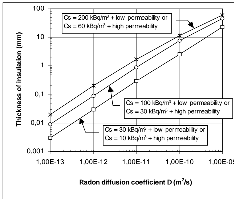
Fig. 4. Thickness of the insulation calculated according to the equation (6) for different values of D and various combinations of soil gas radon concentration and soil permeability. The influence of the soil permeability is introduced by the safety factor \alpha_1 that increases proportionally with the permeability. Chart is valid for the house with habitable rooms in the basement.
