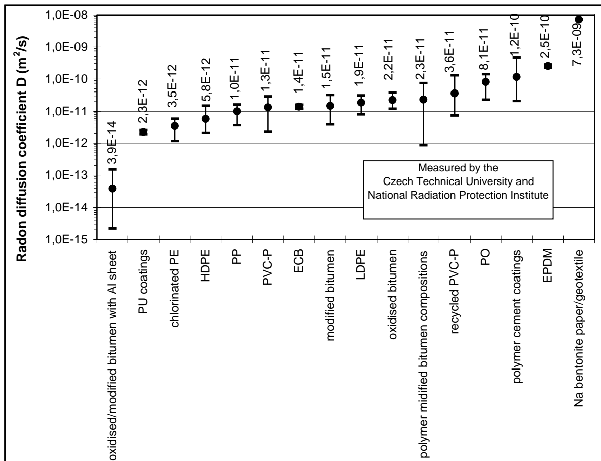
Fig. 3. Summary of the radon diffusion coefficient measurements realized in various waterproofing materials. On x-axis materials are registered with respect to rising order of their diffusion coefficients (HDPE - high density polyethylene, LDPE - low density polyethylene, PVC-P - flexible polyvinyl chloride, PP - polypropylene, PO – polyolefin, PU – polyurethane, ECB - ethylene copolymer bitumen, EPDM - ethylene propylene dien monomer).
